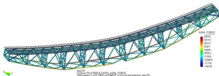
Numerical verification of redundancy against collapse of the steel truss bridge caused by fracture of a member
